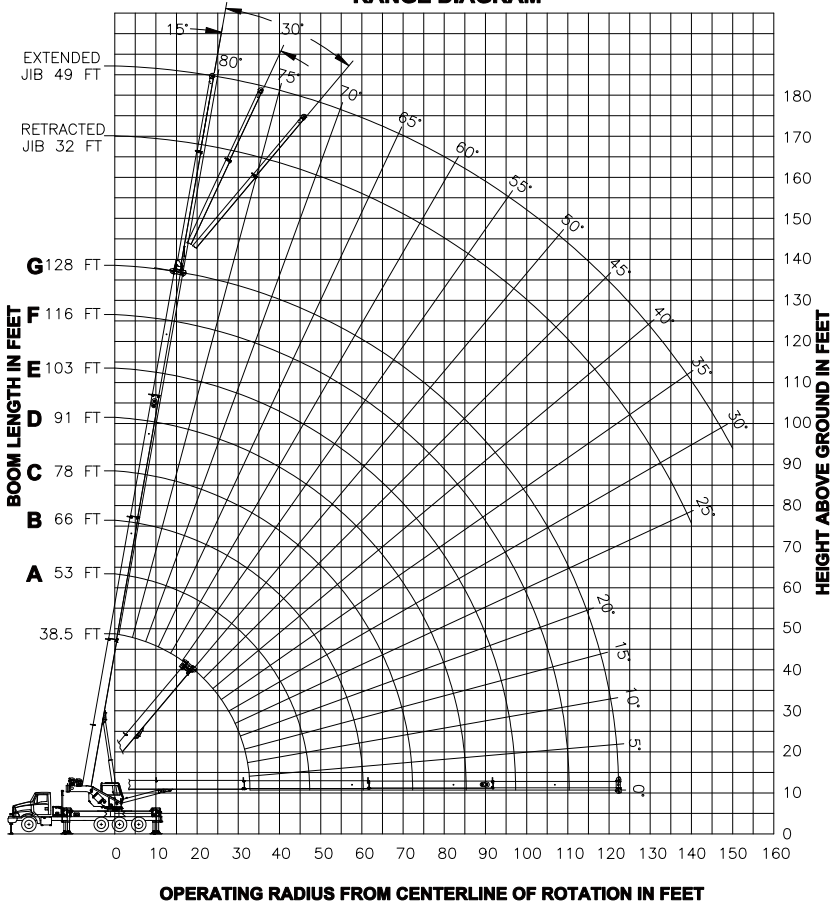
- RANGE DIAGRAM -
