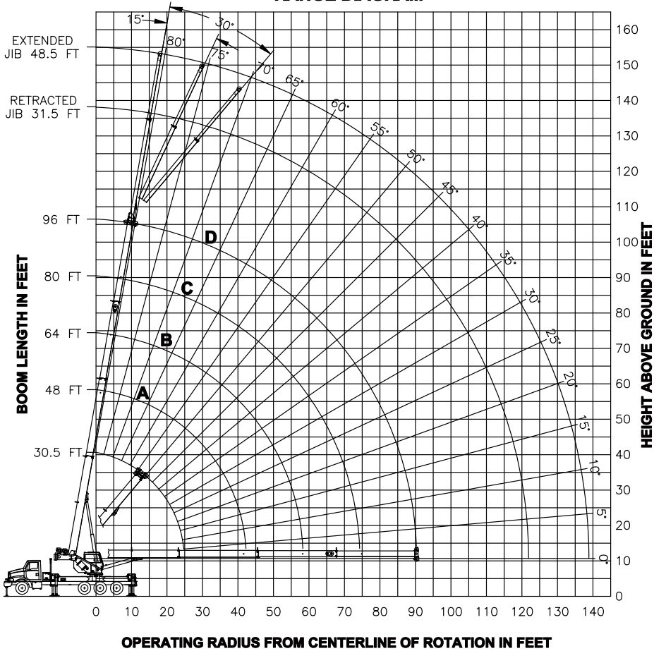
- RANGE DIAGRAM -
